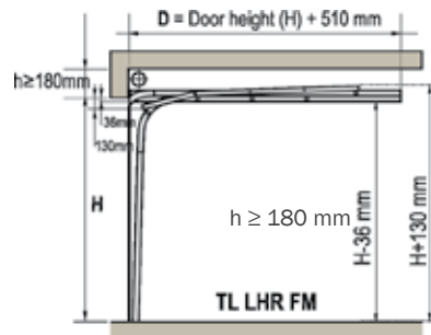
LHR FM low headroom lift double tracks, front mounted springs
