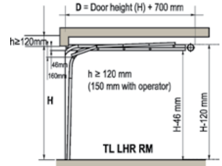
LHR RM low headroom lift double tracks, rear mounted springs
